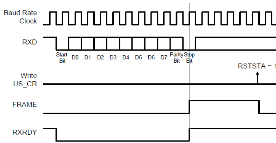
Figure 30-19: Timing Diagram of Frame Error Status
