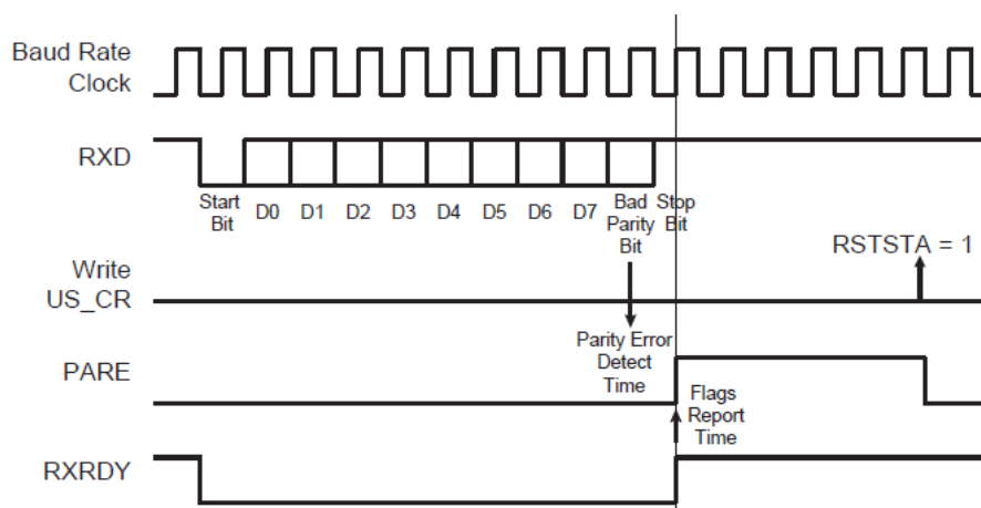
Figure 30-17: Parity Error Timing Diagram
