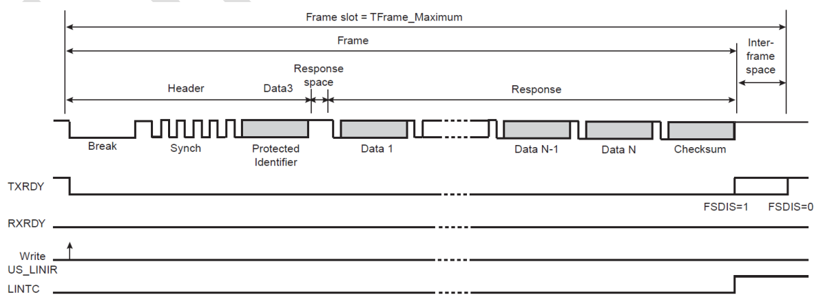
Figure 30-37: Master Node Configuration, NACT = IGNORE
