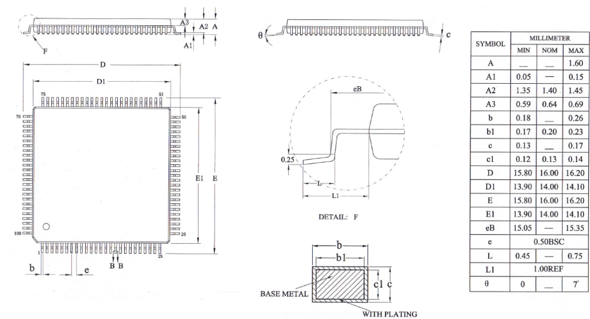
Figure 5-1: LQFP100 Package Outline Drawing
