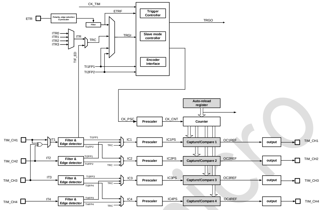
Figure 19-1: System Block Diagram of TIM1–TIM4 & TIM8–TIM13
