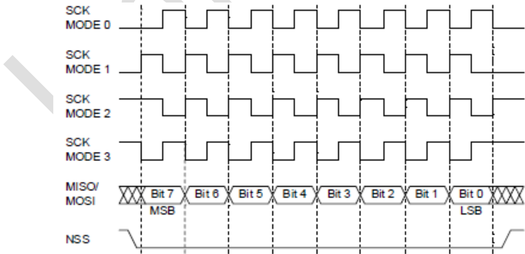
Figure 31-4: Transmission Timing Diagram of SPI in Different Modes in Motorola Mode
