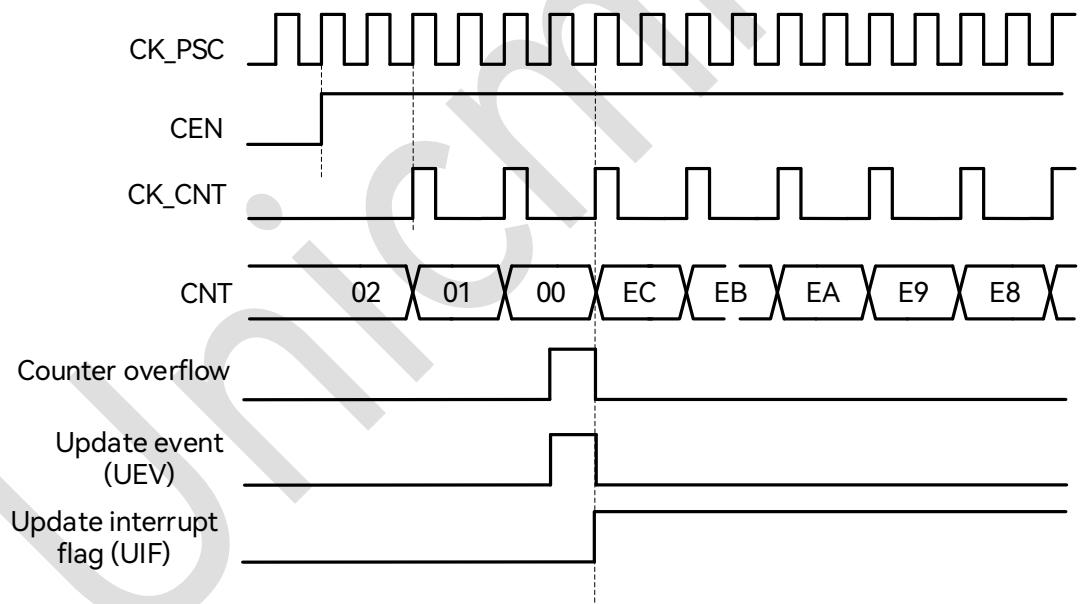
Figure 18-10: Down-counting Waveform Diagram, Internal Clock Divided by 2
