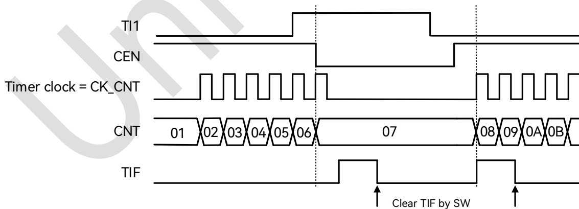
Figure 18-40: Timing Diagram in Gated Mode
