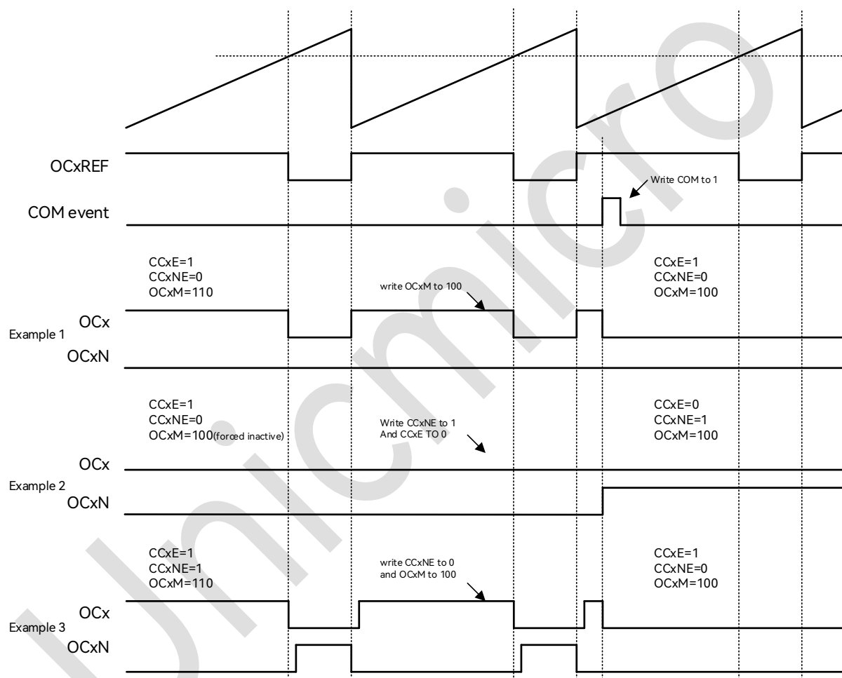
Figure 18-35: 6-step PWM Generation, COM Example (OSSR = 1)
