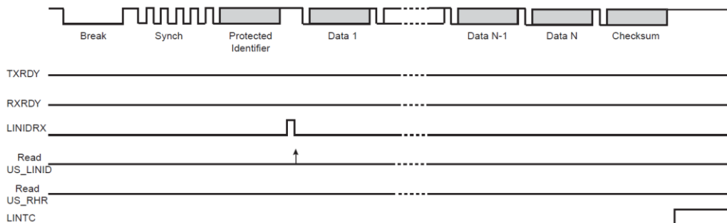
Figure 30-40: Slave Node Configuration, NACT = IGNORE
