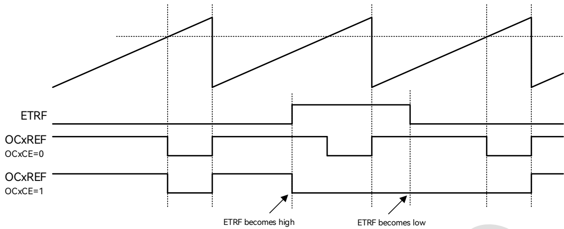
Figure 19-31: ETR Signal Clearing OCxREF of TIM
