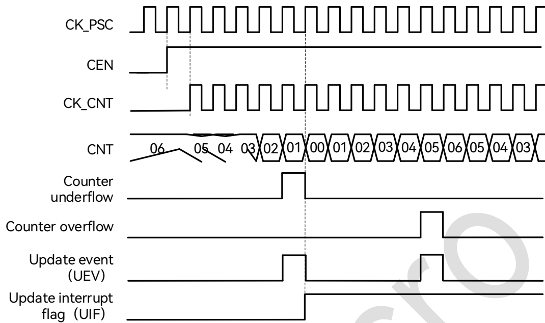
Figure 19-12: Center-aligned Counter Timing Diagram, TIM_PCS = 0, TIM_ARR = 0x6
