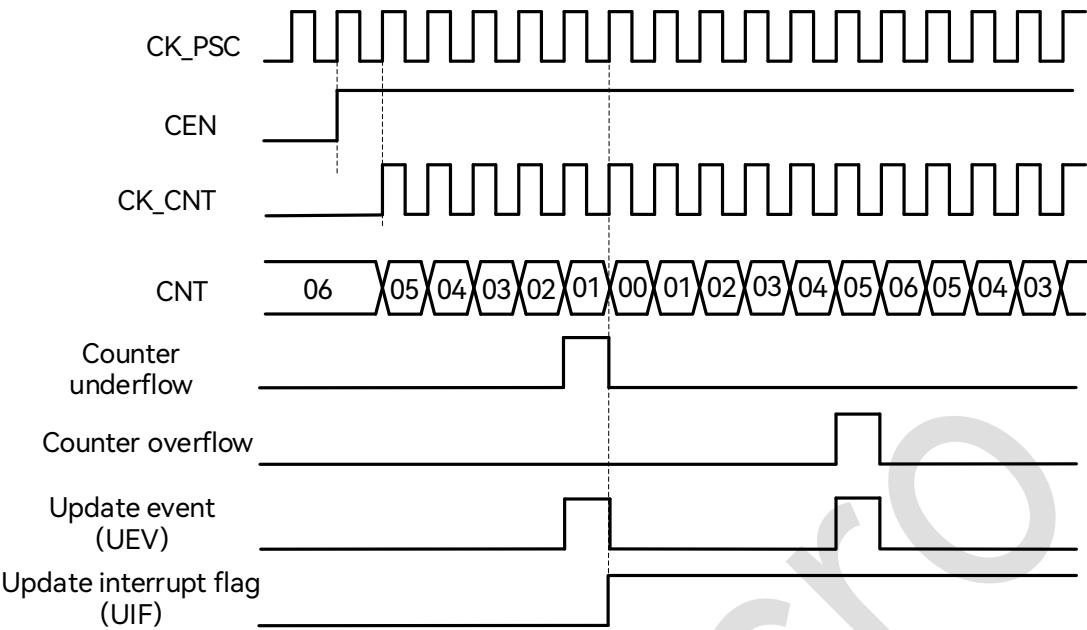
Figure 18-12: Center-aligned Counter Timing Diagram, TIM_PCS = 0, TIM_ARR = 0x6
