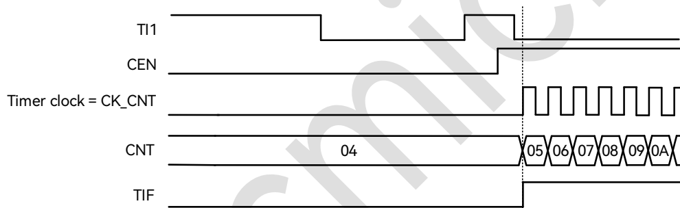
Figure 19-35: Timing Diagram in Trigger Mode
