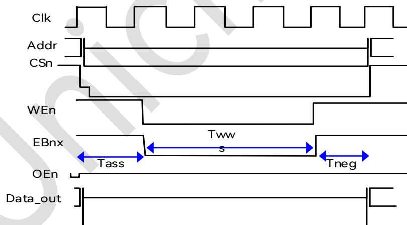
Figure 13-1: Write Operation Timing Diagram for Off-chip Memory Controller
