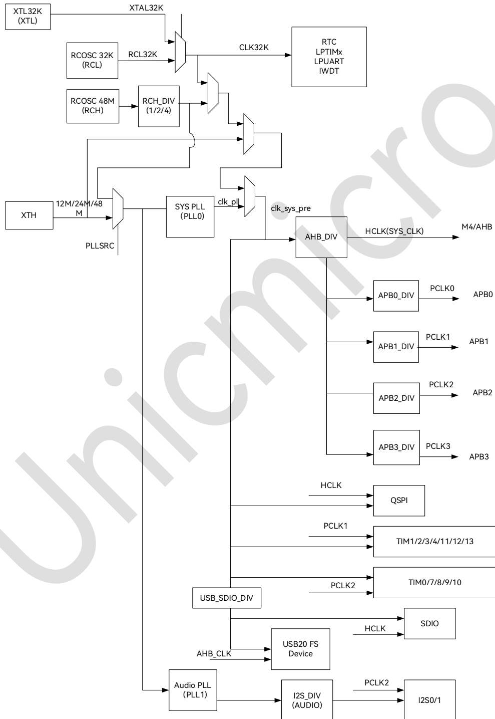
Figure 6-1: Clock Logic
