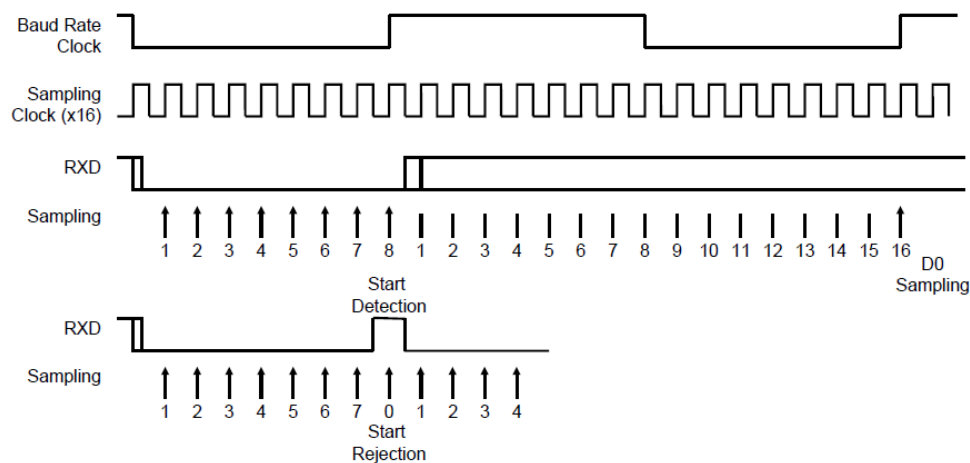
Figure 30-7: Asynchronous Start Bit Detection
