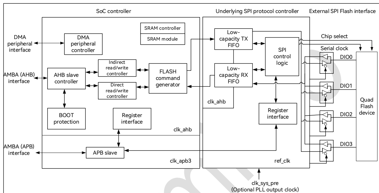
Figure 32-1: QSPI System Block Diagram
