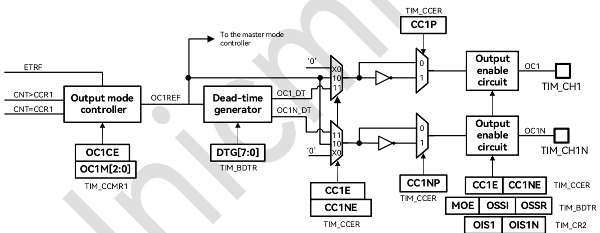
Figure 19-24: Output Stage of Capture/Compare Channel (Channels 1–3)
