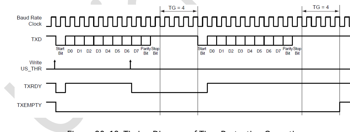
Figure 30-18: Timing Diagram of Time Protection Operation
