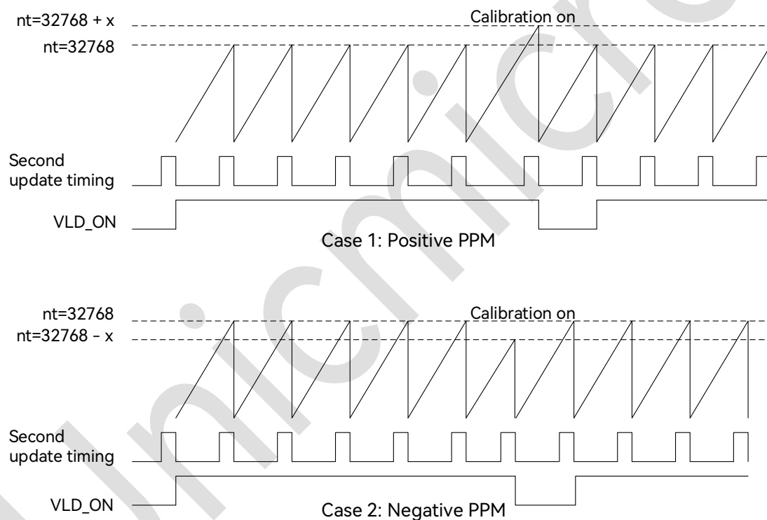
Figure 24-2: Oscillator Calibration
