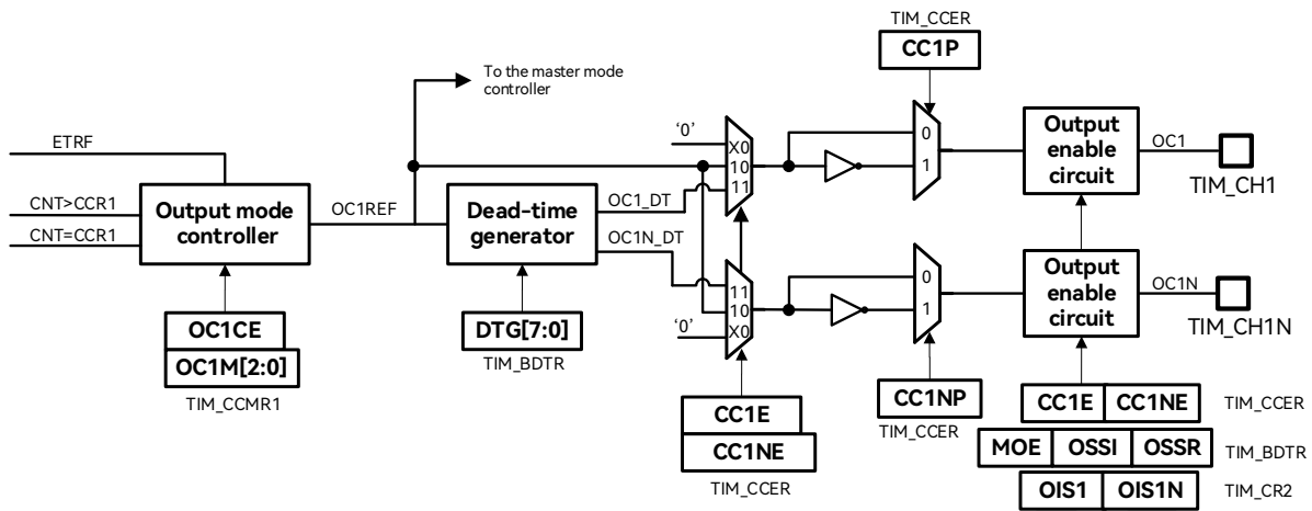
Figure 18-25: Output Stage of Capture/Compare Channel (Channels 1-3)
