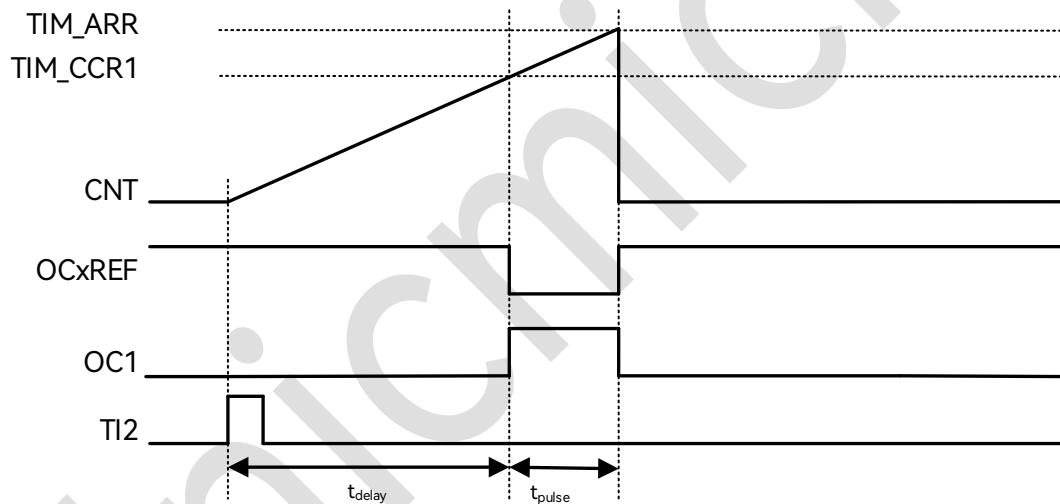
Figure 18-36: Timing Diagram of One-pulse Mode
