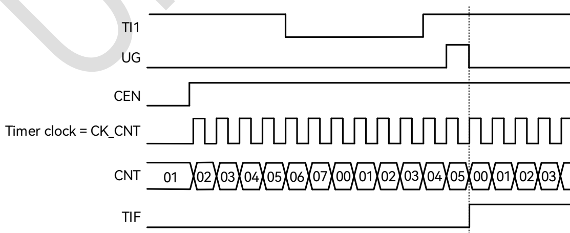
Figure 18-39: Timing Diagram in Reset Mode
