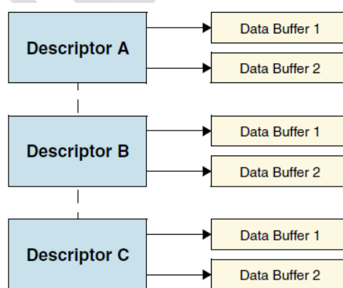
Figure 33-1: Double Buffer Structure Diagram
