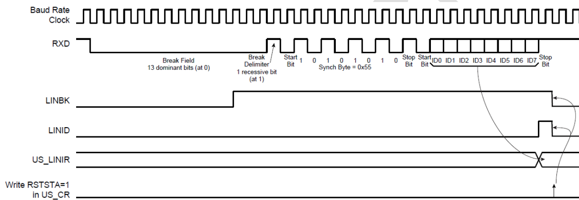
Figure 30-30: Message Reception
