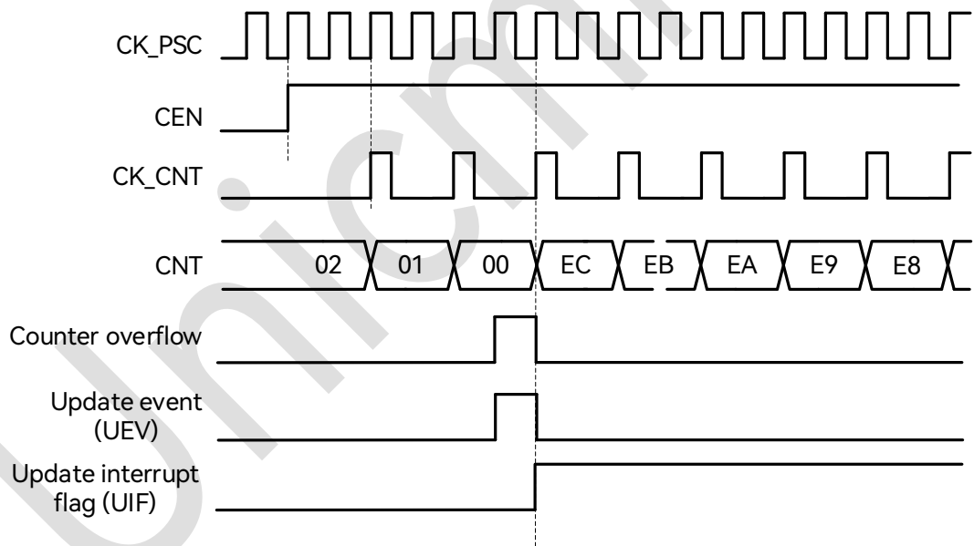
Figure 18-10: Down-counting Waveform Diagram, Internal Clock Divided by 2
