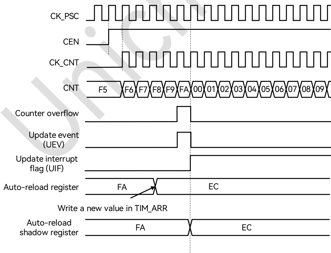
Figure 18-7: Counter Timing Diagram, Update Event when ARPE = 1 (TIM_ARR Preloaded)
