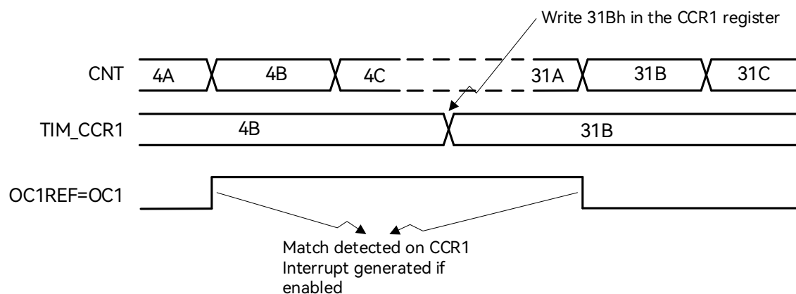
Figure 18-28: Output Compare Mode, Toggle on OC1
