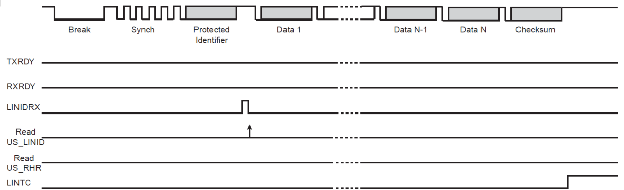
图 30-40: 从节点配置, NACT = IGNORE
