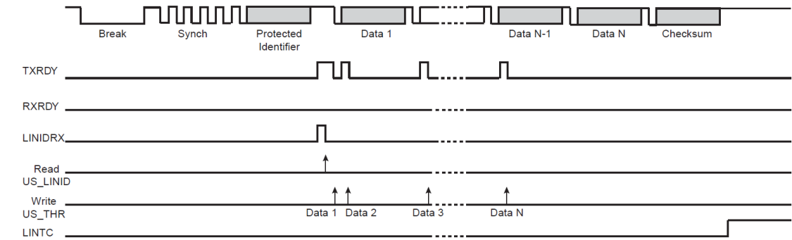
图 30-38: 从节点配置, NACT = PUBLISH
